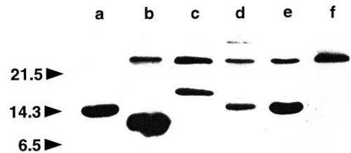
Fig. 3. Strep-tagged proteins in the cytoplasm of cytochrome c -producing cells. E. coli BL21 (DE3) cells were used to coexpress various combinations of cytochromes and yeast cytochrome c heme lyase. Bacterial lysate comprising approximately 20 µg of protein were run on SDS–PAGE and blotted onto nitrocellulose membranes. Membranes were then decorated with streptavidin–peroxidase conjugate and StrepTags were visualized according to the manufacturer's recommendations (IBA, Göttingen). The strongly staining band at 22 kDa which shows up in all cell lysates probably represents the E. coli biotin carboxyl carrier protein, which was decorated despite preincubation of the lysates with avidine). Lane a, purified iso -2-cytochrome c (Cyc7) as in Fig. 2, lanes g and h; b, PetJ; c, CycA; d, Cyc1; e, Cyc7; and f, plasmid pET-3a without insert.
